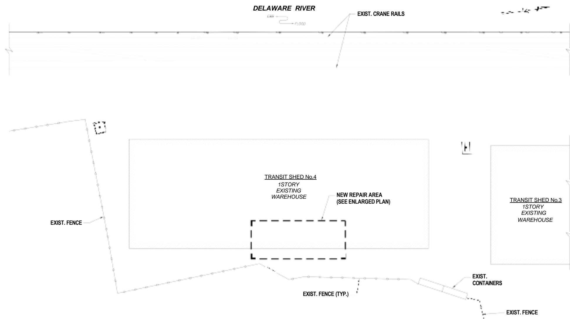
SITE PLAN SCALE 1"=50'
