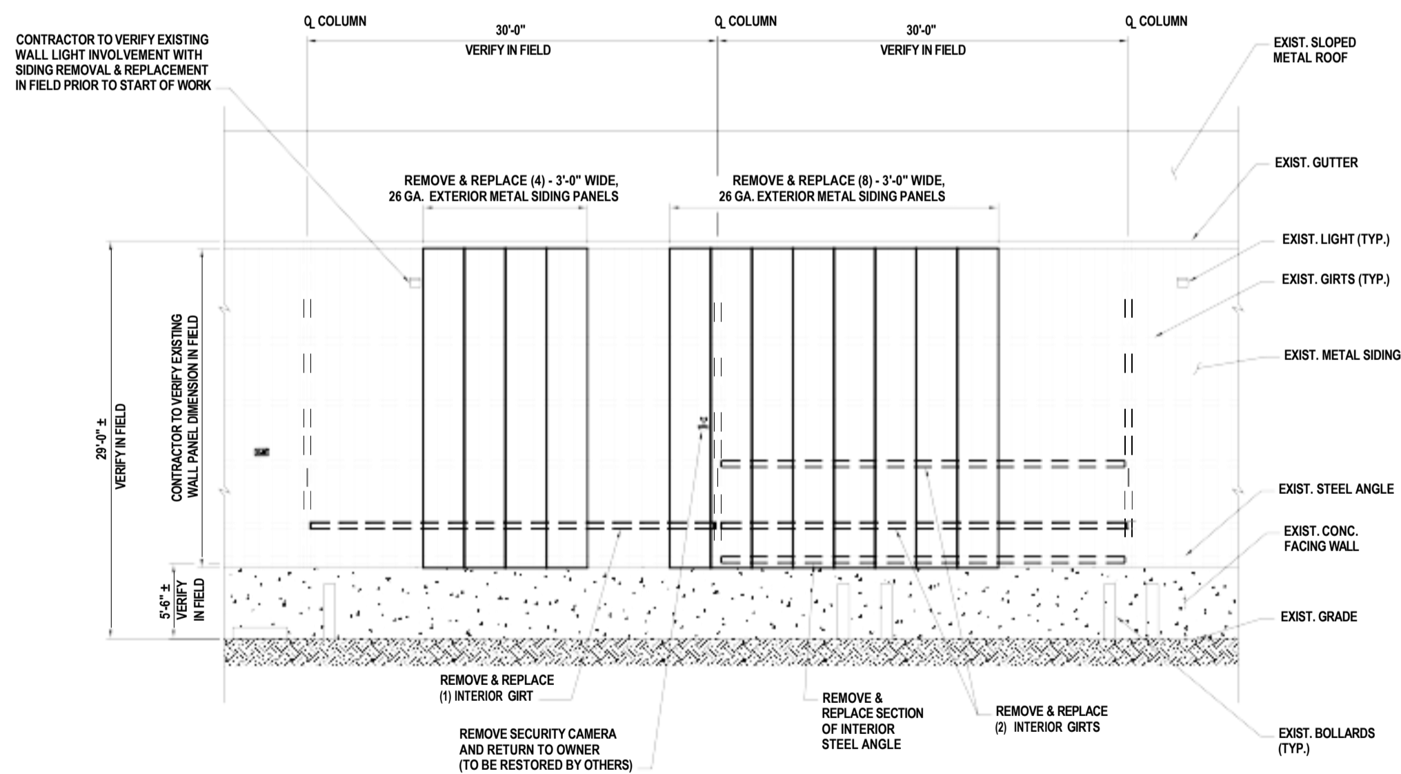
EXTERIOR ELEVATION SCALE 1/8"=1'-0"
