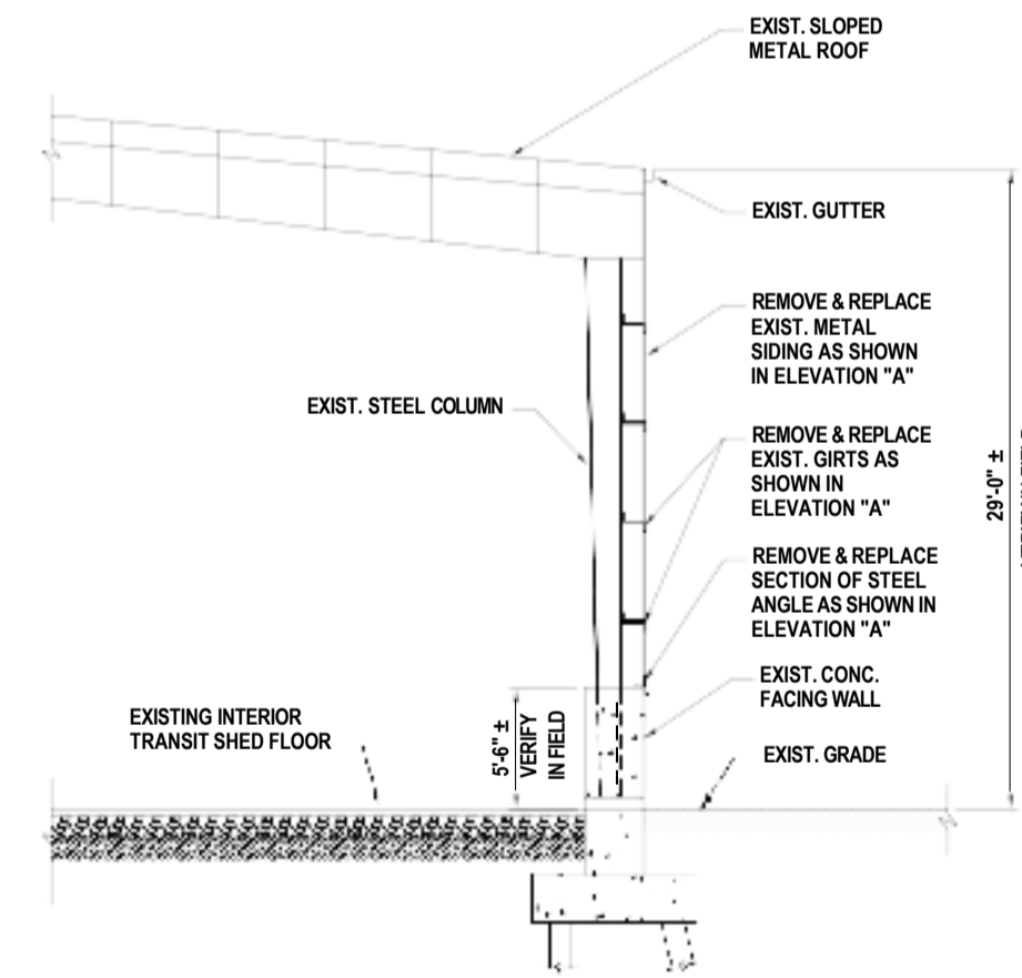
SECTION SCALE 3/8"=1'-0"
