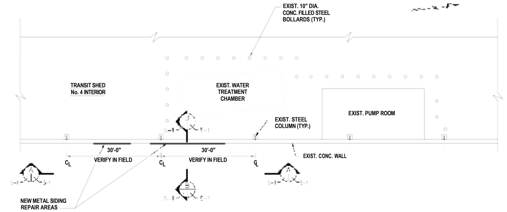
ENLARGED PLAN SCALE 1"=10'
