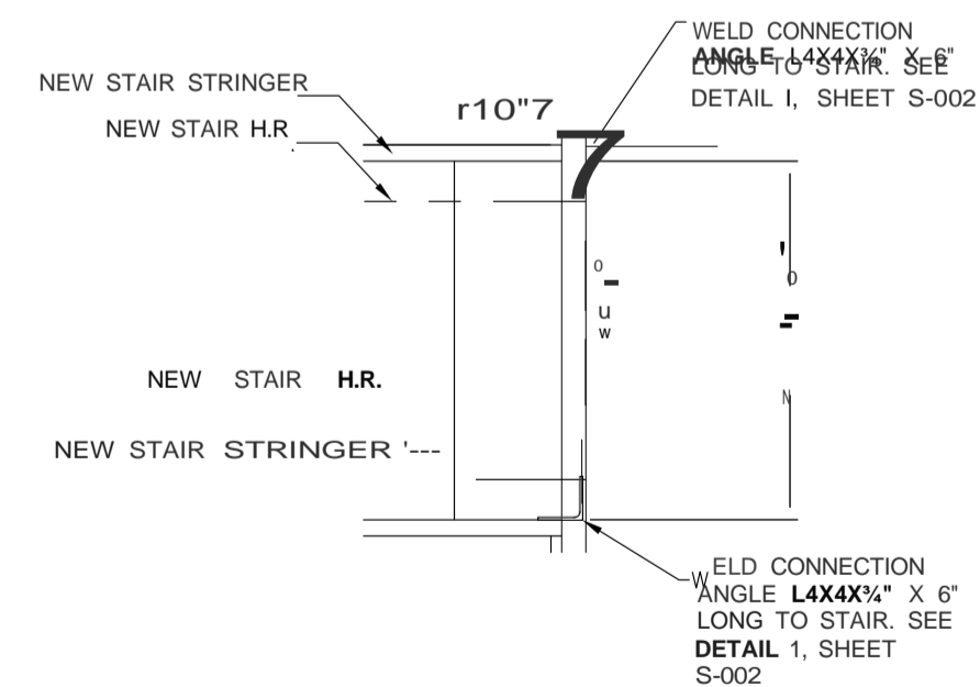
ENLARGED PLAN SCALE: 1" = 1'-0"
