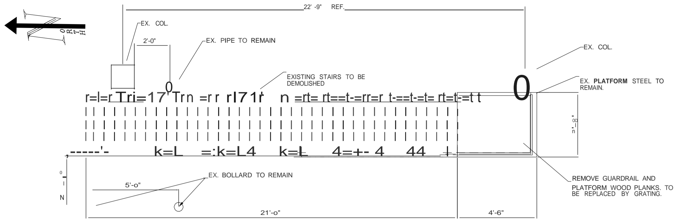
EXISTING STAIRS DEMO PLAN SCALE: 1/2" = 1'-0"
